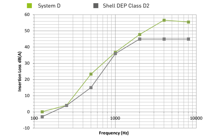
Test results acc. to Shell DEP 31.46.00.31-Gen.
